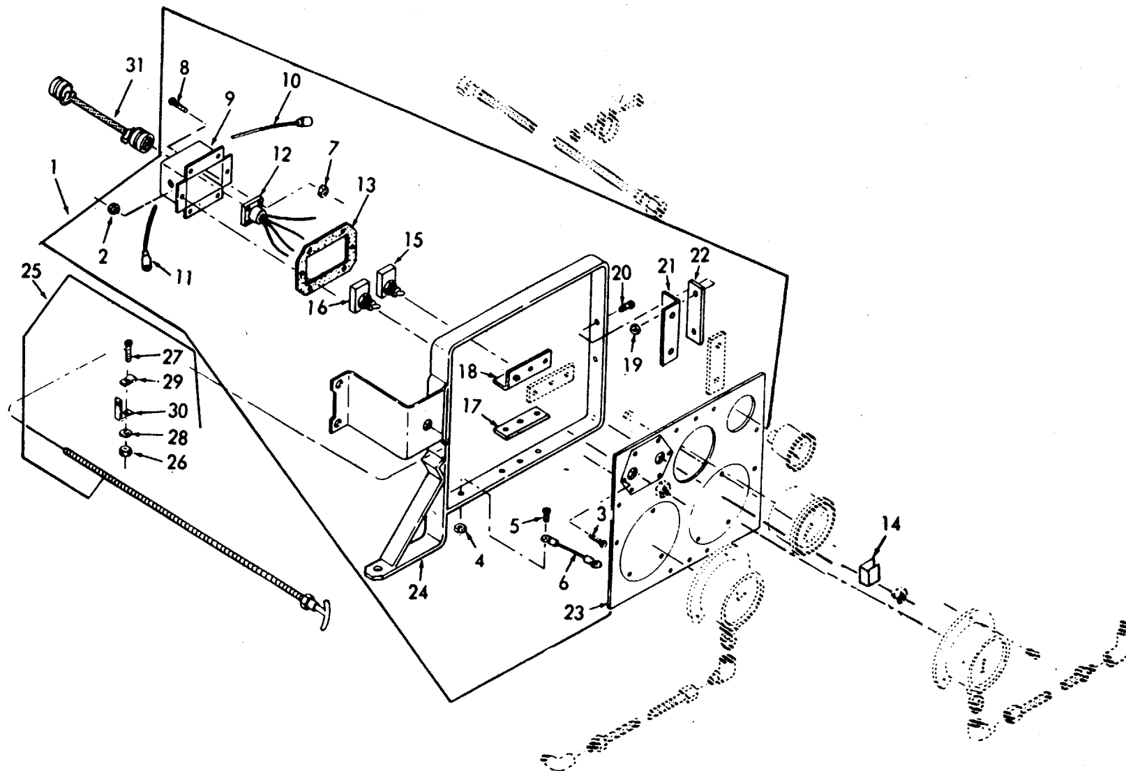
Figure 7. Control Panel.
