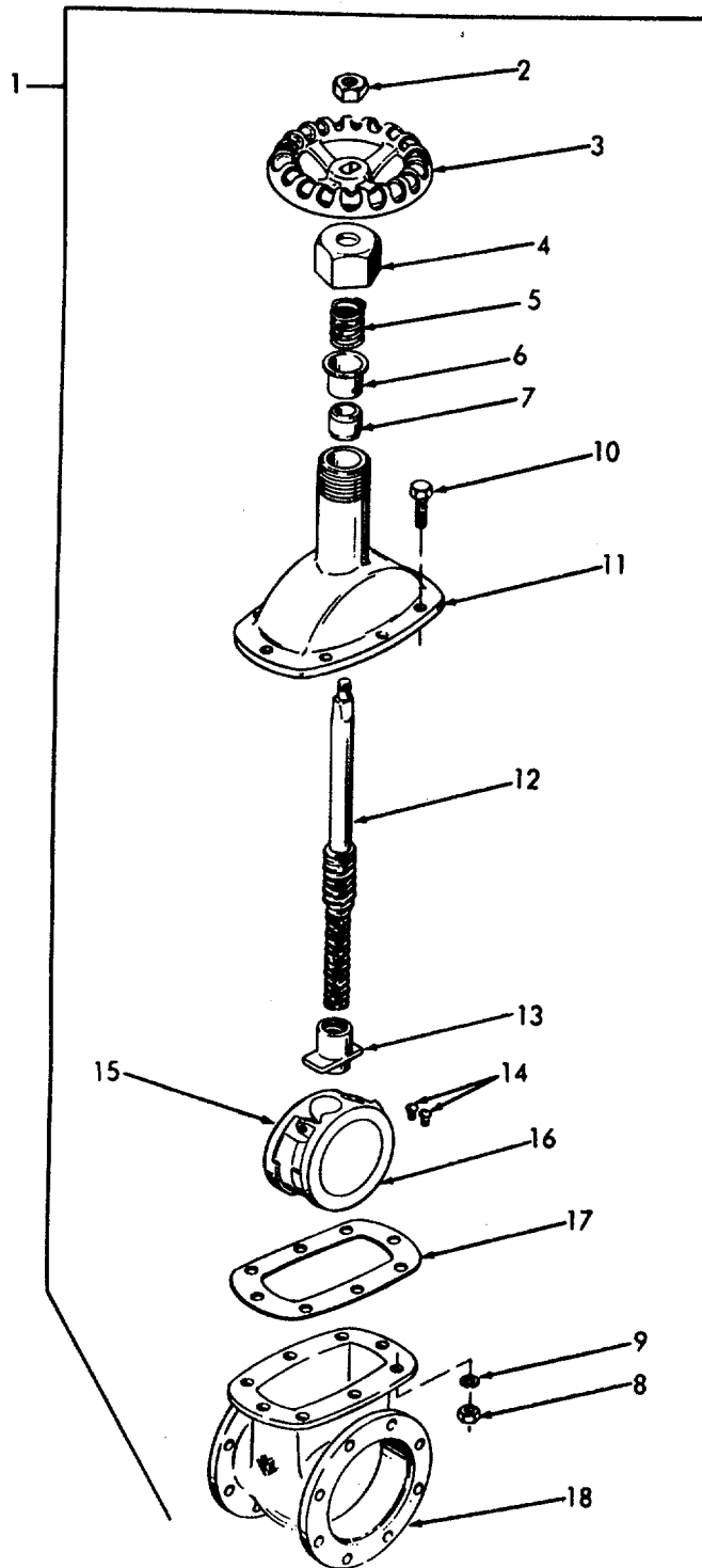
Figure 9. Gate Valve.
