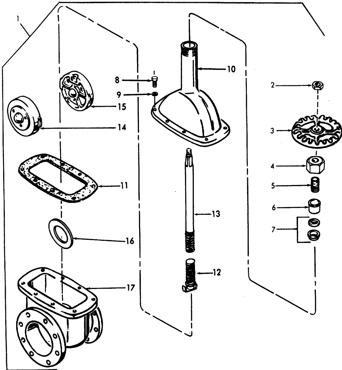
Figure 8. Gate Valve.
