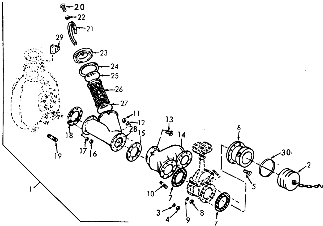
Figure 11. Strainer.
